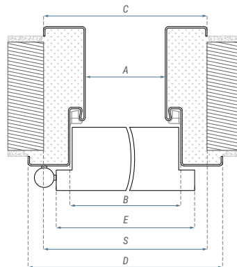
Dimensions of BORD fixed door frame [mm]:
